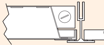
CRI 2" Walkable Grid 24 1/2" x 48 1/2" o.c.
